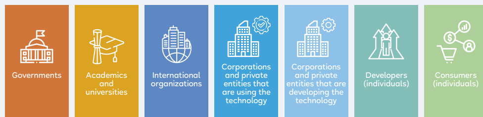
Figure 03 Quantum computing stakeholders (Source: World Economic Forum)
