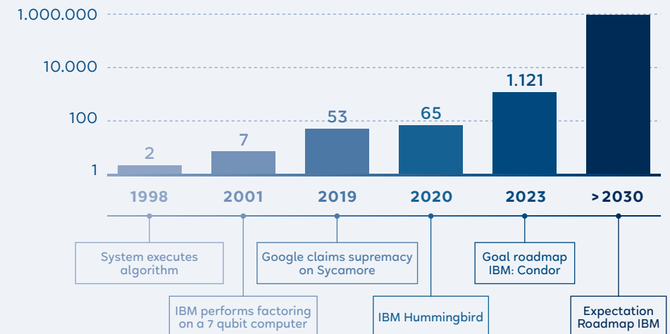
Figure 08 Number of qubits in in quantumcomputers (>10.000 qubits are needed for simple applications). Source: Birch (2021)
